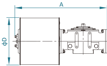
Fig.545 Air/air (Double acting)
