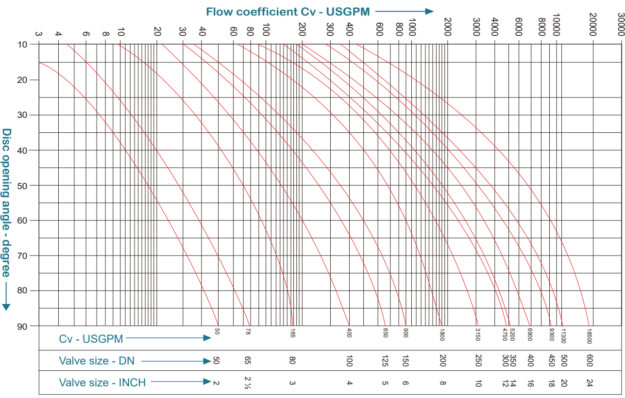
Cv curve - Class300, PN25/40 valves
