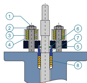
Live-loaded packing system
