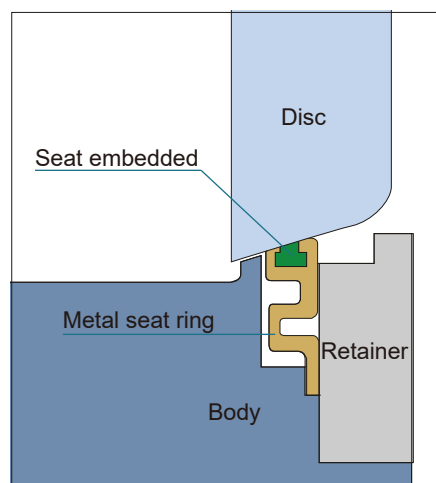
During fire and after fire
