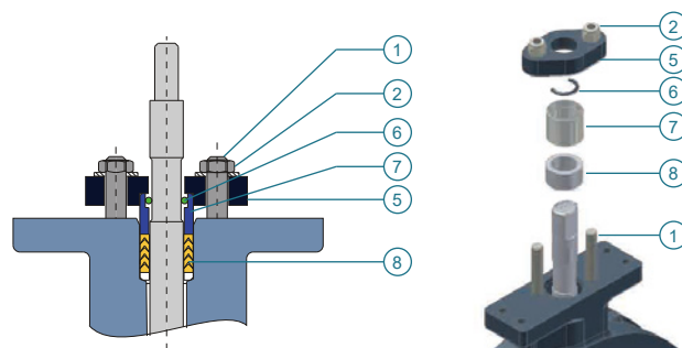
Packing sealing system Standard
