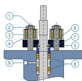
Double-packed live-loaded Monitoring port optional
