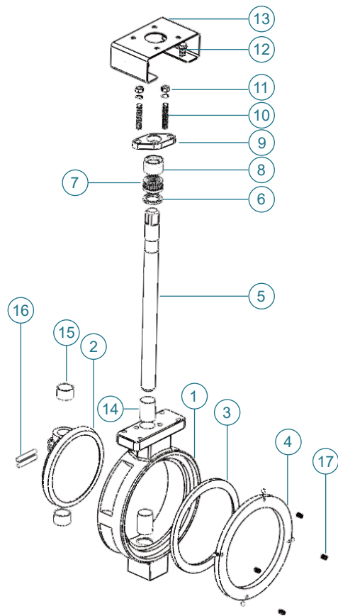
Wafer type
