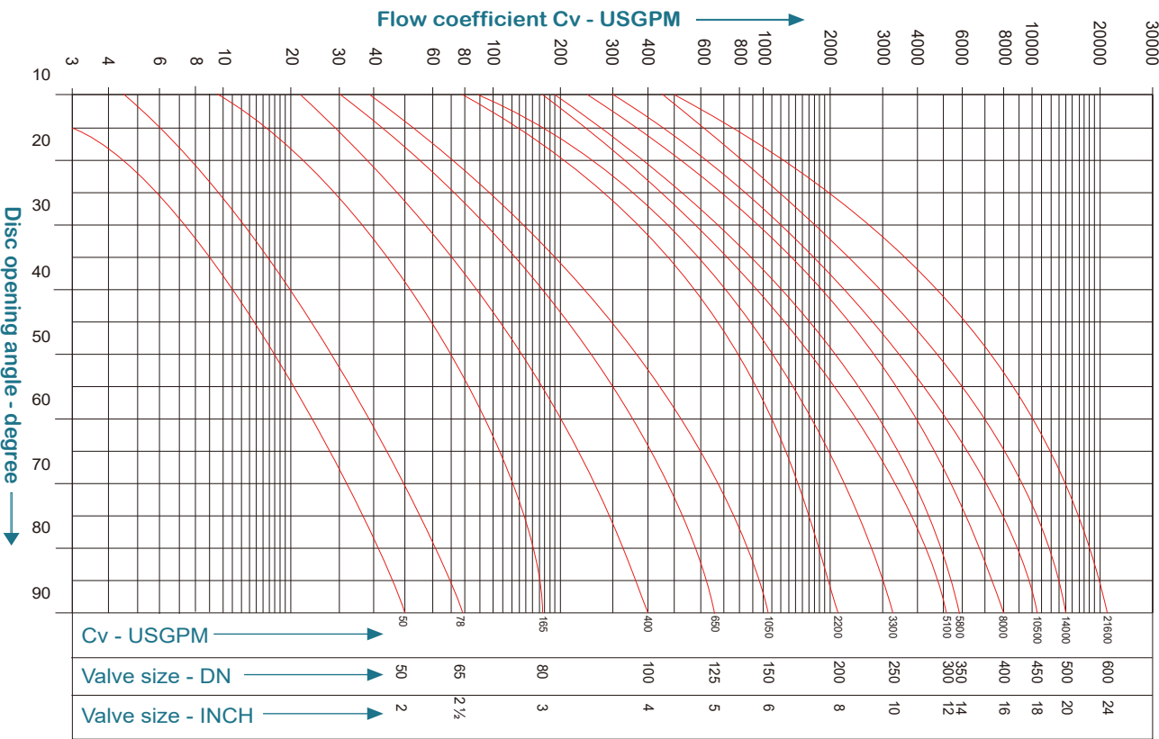
Cv curve - Class150, PN10/16 valves
