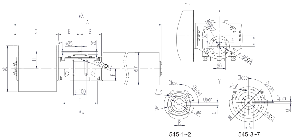
Dimensions - Spring return
